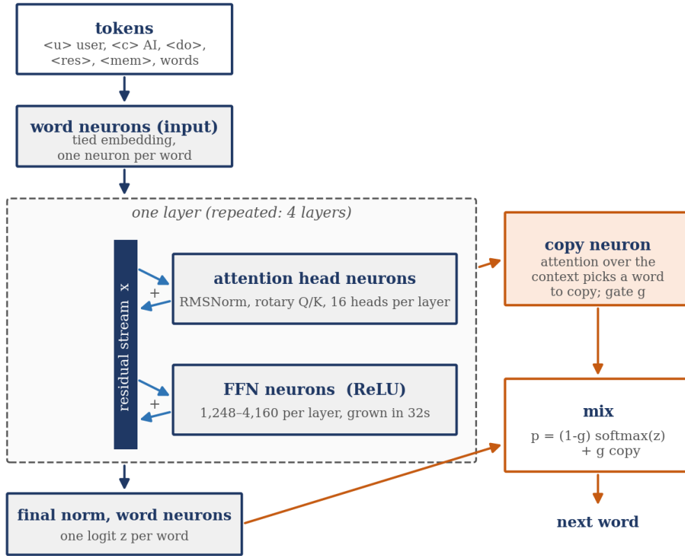
Figure 3. The neural brain. Head and FFN neurons add into the residual stream x . The copy neuron mixes a pointer distribution into the output.
